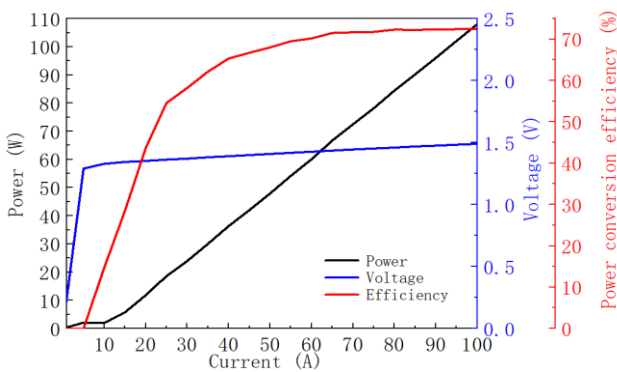
Power-Current-Voltage-Efficiency
